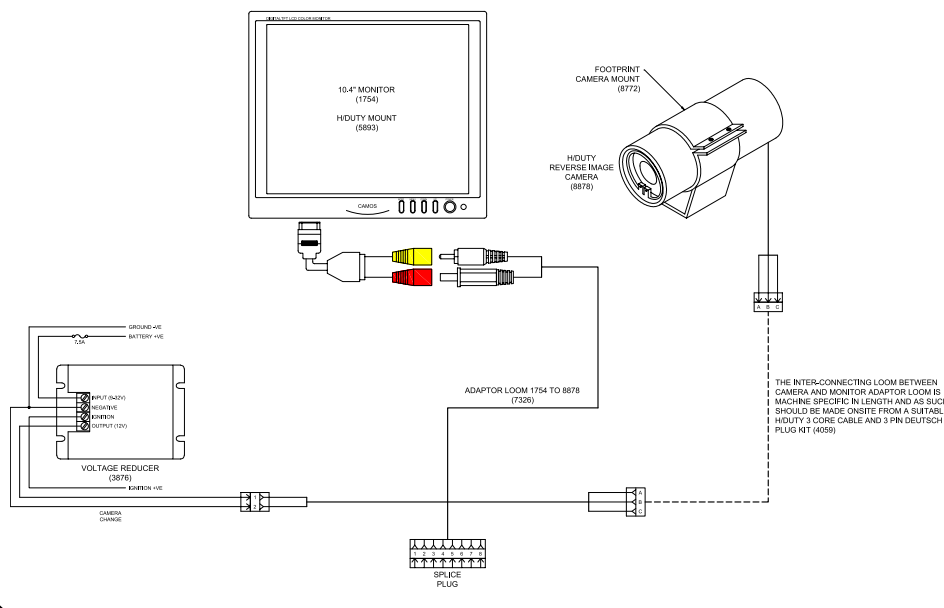
1754 MONITOR COLOUR LCD TFT 10.4" MONITOR WITH 8878 REVERSE IMAGE CAMERA
